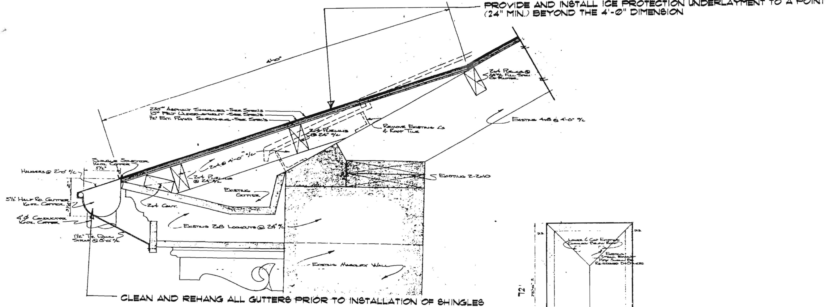
EXISTING ROOF SECTION NO SCALE
