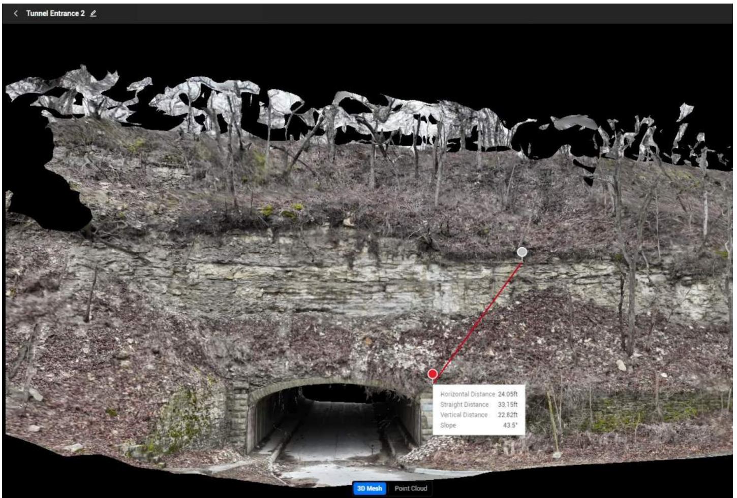
NE Bluff Right Side Dimension
