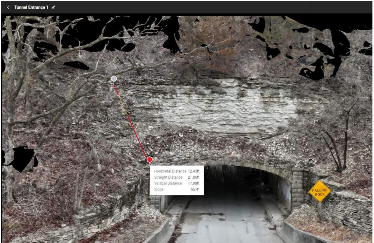
SW Bluff Left Side Dimension
