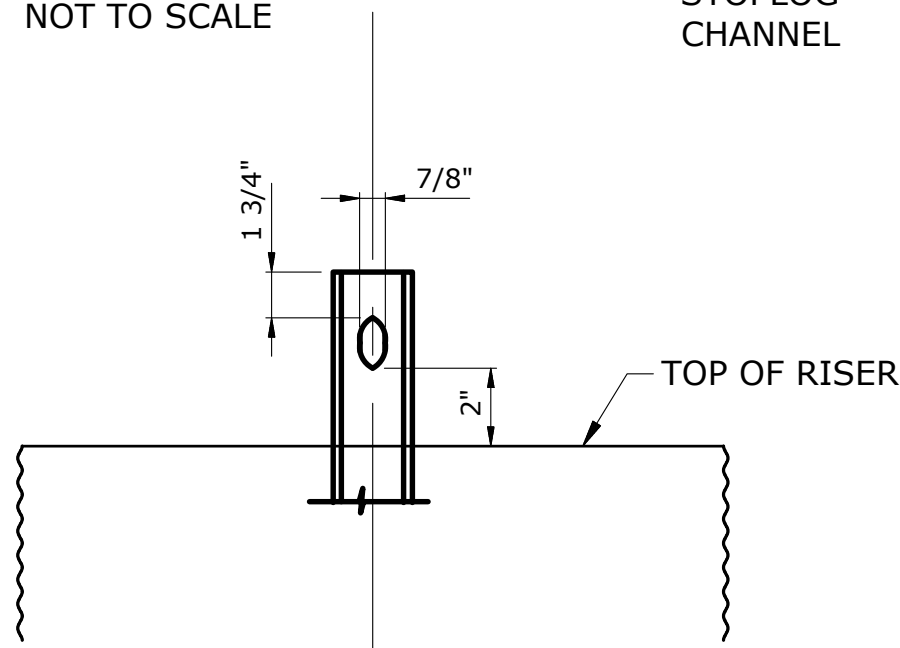
LOCKING ROD SLOT DETAIL NOT TO SCALE
