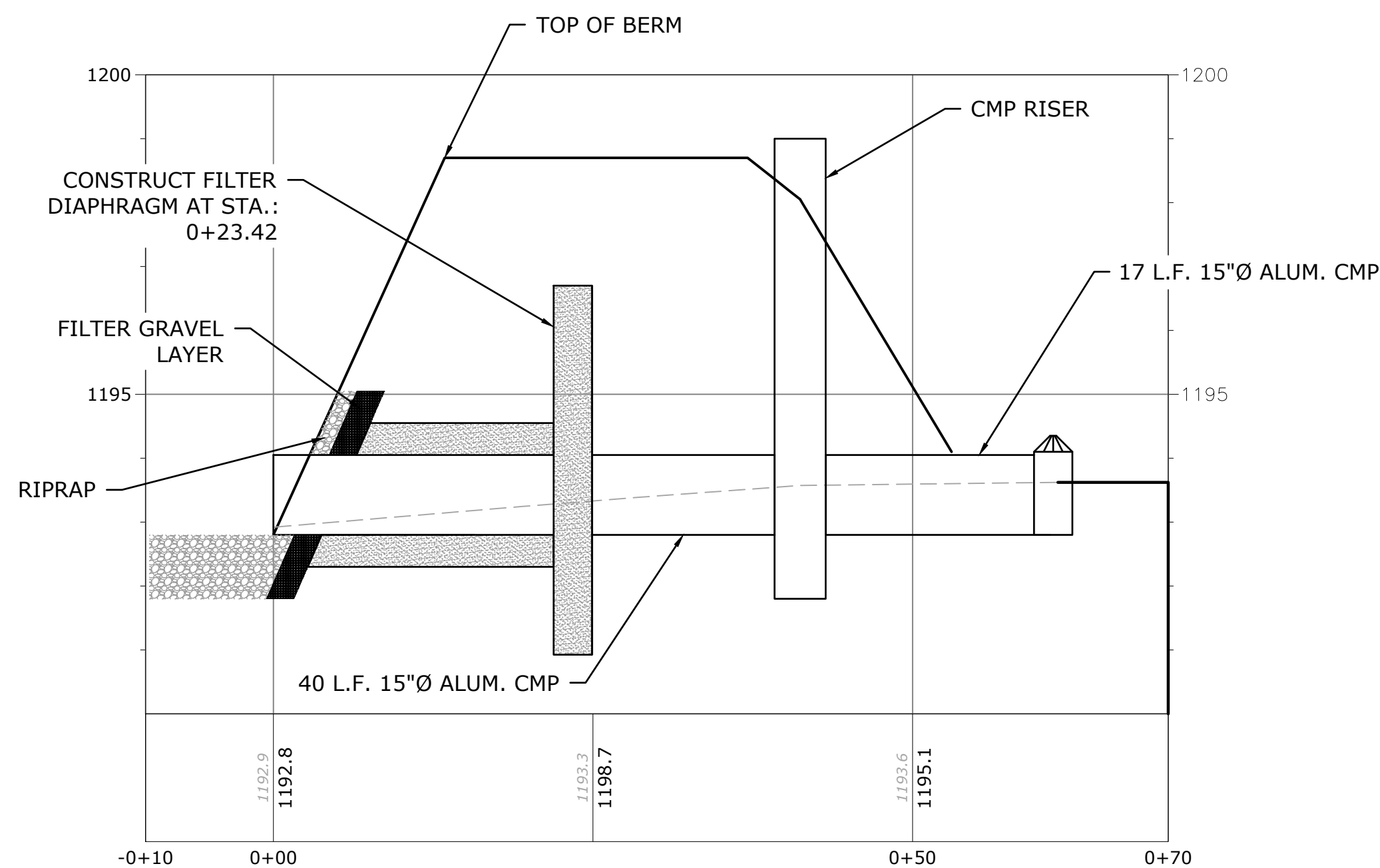
PLAN - FILTER DIAPHRAGM
