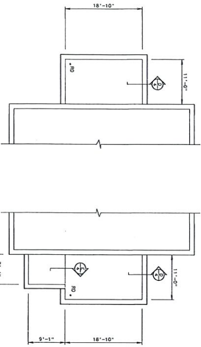
ROOF PLAN - ELEMENTARY SCHOOL SCALE: 1/8" = 1'-0"
