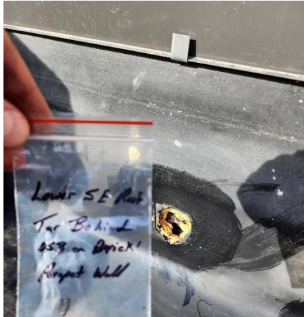
Photo #7 Sample #24. Asbestos containing tar. Lower southwest and northwest roofs, behind OSB on brick parapet wall.
