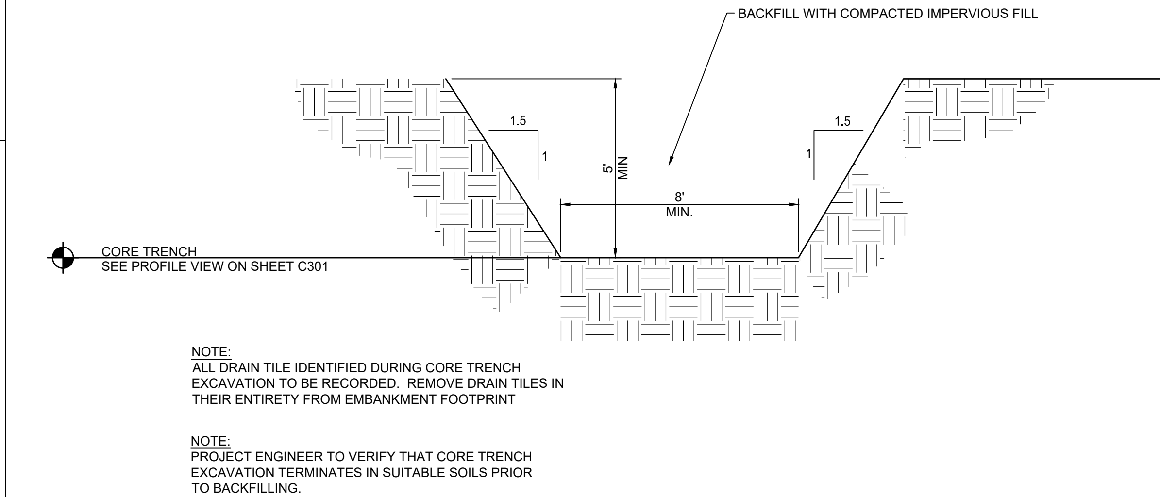
A4 TYPICAL CORE TRENCH SECTION NOT TO SCALE
