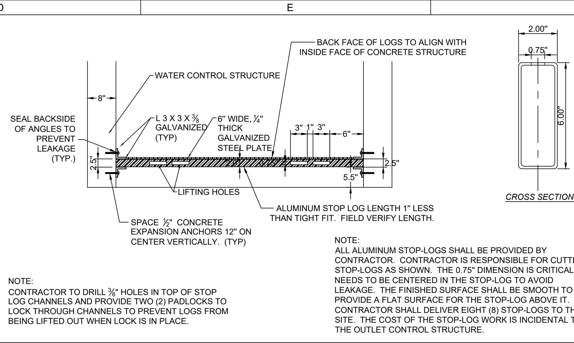
D1 STOP LOGS AND CHANNEL NOT TO SCALE
