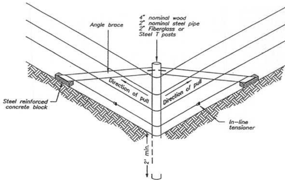
Single Post Corner or Angle Brace Assembly
